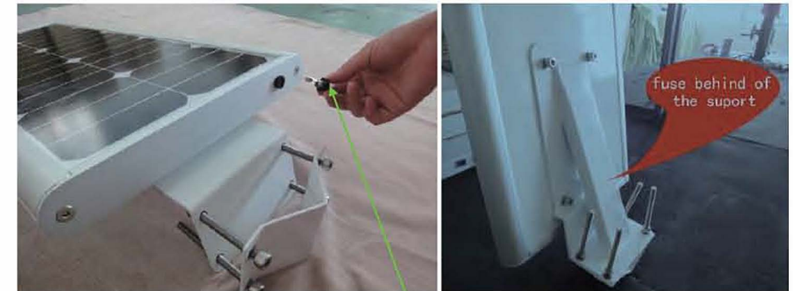
Step 5: Insert the fuse into the light fixture/box. Unfold the knob of fuse (see below) and take out the insulating film of the fuse socket. Make sure the fuse is working, then tighten.
